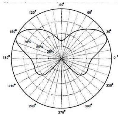
3D Spatial Radiation Pattern
