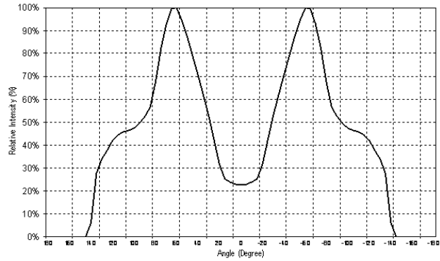
Vertical Spatial Radiation Pattern
